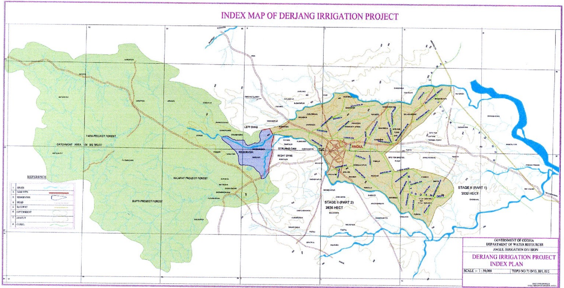
Index Map of Derjang Irrigation Project
